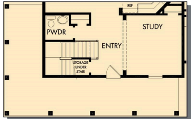
First Floor with Optional Wrap Around Porch
